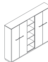
X5119 2496 / 421 / 1871 302.7 kg
